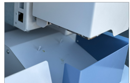
Improved glue applicator, always with closed tank, suitable for EVA and PUR glue.
