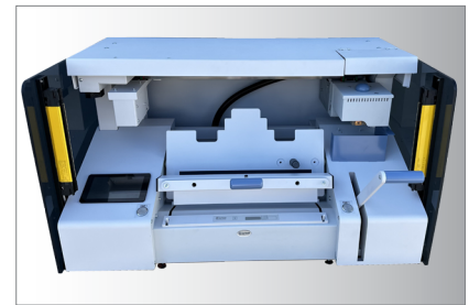
PUR/EVA perfect binder
